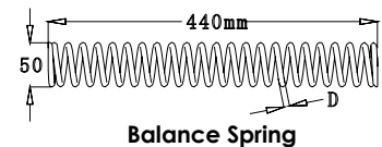
Parameter of Balance Spring Diameter Selection
